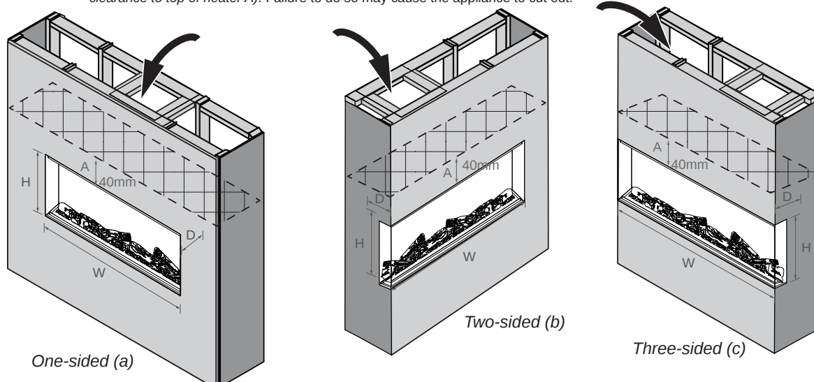
Figure 4. Cavity Dimensions
