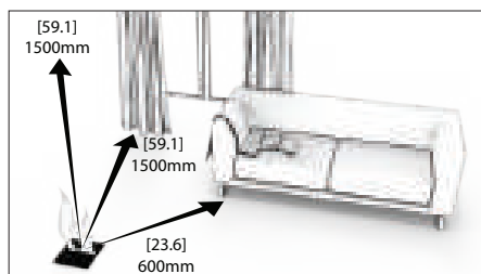
Indoor Clearances
