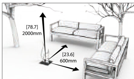
Outdoor Clearances
