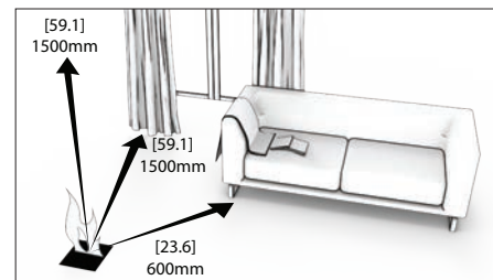
Indoor Clearances
